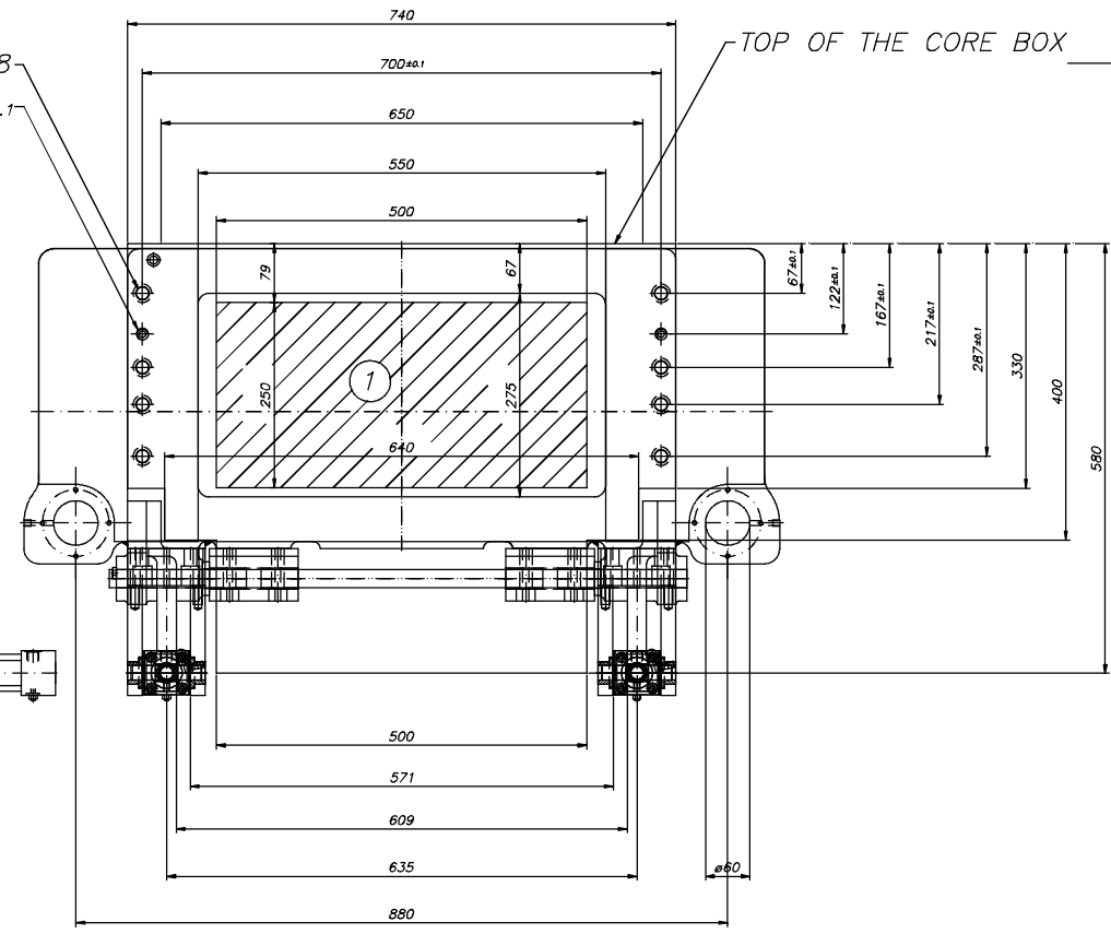
1 EJECTORS PLATE ACTIVATED BY HYDRAULIC CILINDER
