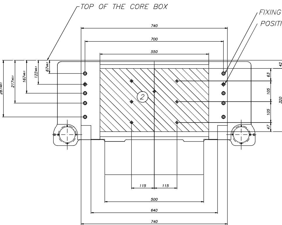
2 EJECTORS PLATE ACTIVATED BY SPRINGS
